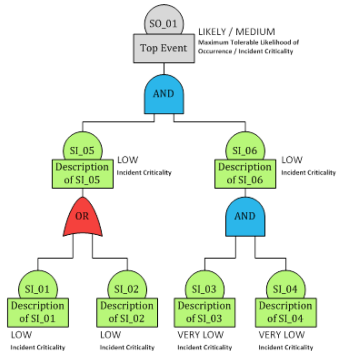
Figure 1. Example of an Attack Tree Analysis
